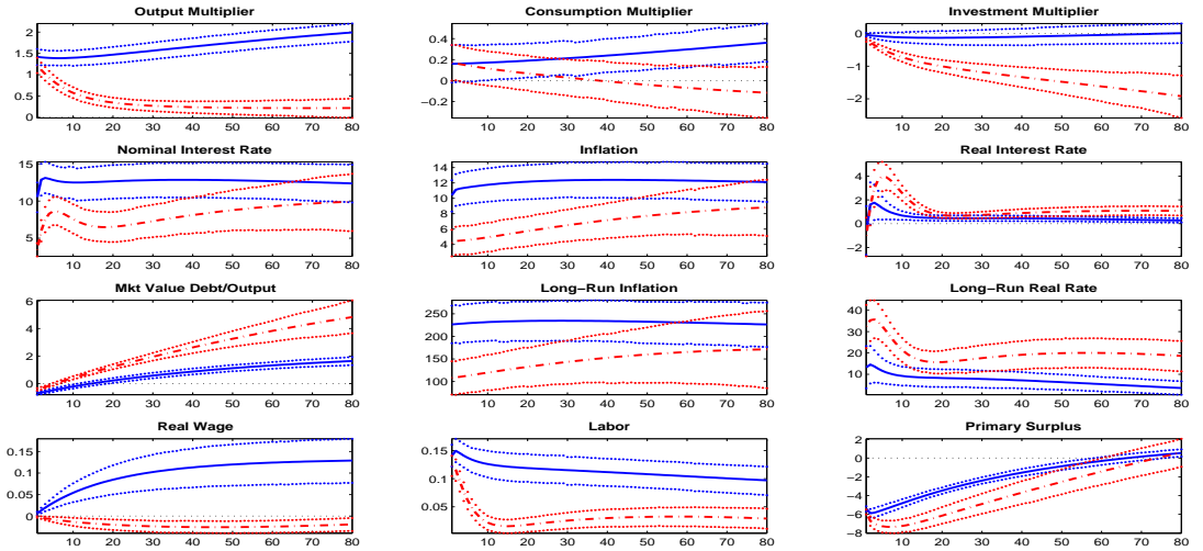
Figure 3: Responses over 80 quarters to a government spending increase in estimated regime M (dashed lines) and regime F (solid lines) over period 1955q1–2007q4. Responses displayed are for the posterior mean parameters and the 90-percent impulse response credible intervals. Top panels are present value multipliers for output, consumption and investment, interest rates and inflation rates are converted to annualized basis points, and the remaining variables are in percentage deviations from steady state.
