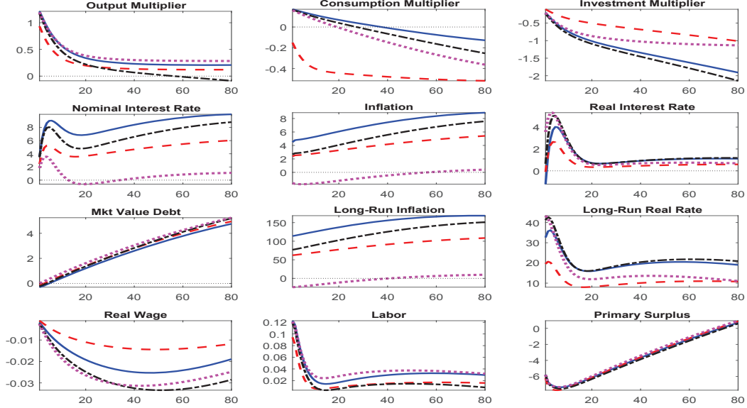
Figure 5: Counterfactual posterior mean responses to a government spending increase in estimated regime M, 1955q1–2007q4. Baseline estimates (solid lines); lower habits, \theta = 0.8 and no government spending in utility, \alpha_G = 0 (dashed lines); more aggressive monetary policy, \phi_\pi = 1.5 and \phi_y = 0.2 (dotted-dashed lines); Ricardian model, \gamma_G = 0, \gamma_Z = 0.2 (dotted lines). Top panels are present value multipliers for output, consumption and investment, interest rates and inflation rates are converted to annualized basis points, and the remaining variables are in percentage deviations from steady state.
