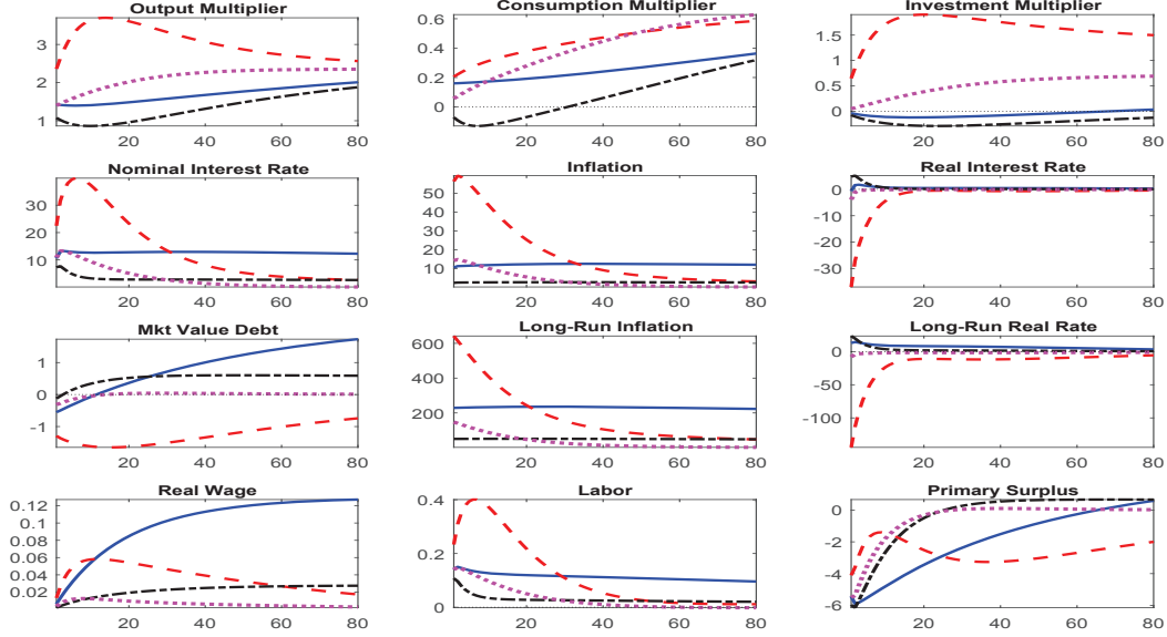
Figure 6: Counterfactual posterior mean responses to a government spending increase in estimated Regime F, 1955q1–2007q4. Baseline estimates (solid lines); lower nominal rigidities, \omega_p = \omega_w = 0.7 (dashed lines); lower habits, \theta = 0.8 , no government spending in utility, \alpha_G = 0 , and less persistent spending shock, \rho_G = 0.9 (dotted-dashed lines); lower nominal rigidities, \omega_p = \omega_w = 0.7 , lower habits, \theta = 0.8 , no government spending in utility, \alpha_G = 0 , and less persistent spending shock, \rho_G = 0.9 (dotted lines). Top panels are present value multipliers for output, consumption and investment, interest rates and inflation rates are converted to annualized basis points, and the remaining variables are in percentage deviations from steady state.
