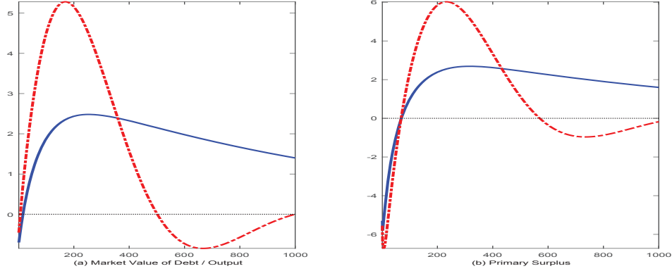
Figure 4: Responses of debt and primary surplus to a government spending increase in estimated regime M (dashed lines) and regime F (solid lines) over period 1955q1–2007q4. Responses displayed are for the posterior mean parameters and variables are in percentage deviations from steady state.
