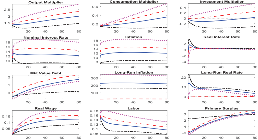
Figure 7: Counterfactual posterior mean responses to a government spending increase in estimated Regime F, 1955q1–2007q4. Baseline estimates (solid lines); only one-period debt, \rho = 0 (dashed lines); higher steady state debt-GDP ratio, s^b = 150 percent (dotted-dashed lines); steady-state tax rates reduced by 40 percent (dotted lines). Top panels are present value multipliers for output, consumption and investment, interest rates and inflation rates are converted to annualized basis points, and the remaining variables are in percentage deviations from steady state.
