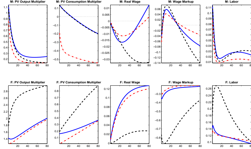
Figure 8: Counterfactual labor market responses to a government spending increase in regime M (top row) and F (bottom row) calibrating both regime using regime F estimates over 1955–2007. Regime M replaces monetary and fiscal parameters with their regime M estimates ( \phi_\pi = 1.14 and \gamma_G = 0.21 ). Reference case (solid lines); reduced habits and eliminating complementarity of government spending, \theta = 0.8 and \alpha_G = 0 (dotted-dashed lines); reduced price rigidities, \omega_p = 0.7 (dashed lines).
